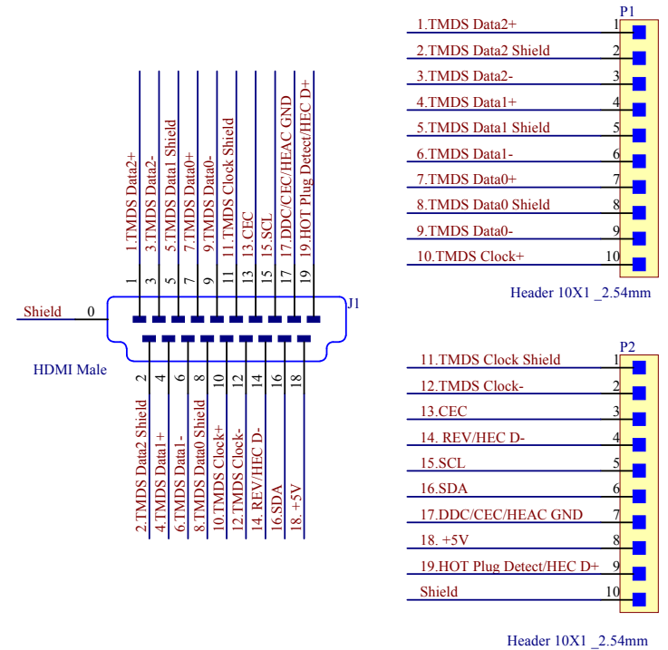
HDMI-AM-BO-V1B Schematic Diagram
