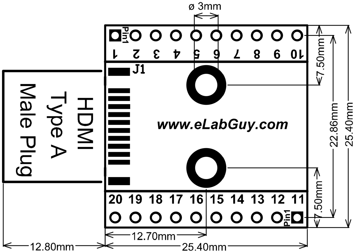
HDMI-AM-BO-V1B PCB outline Drawing
